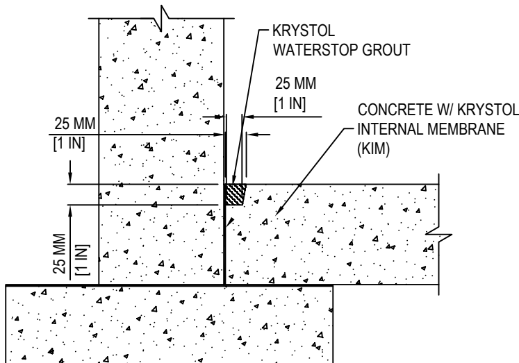
INBOARD
