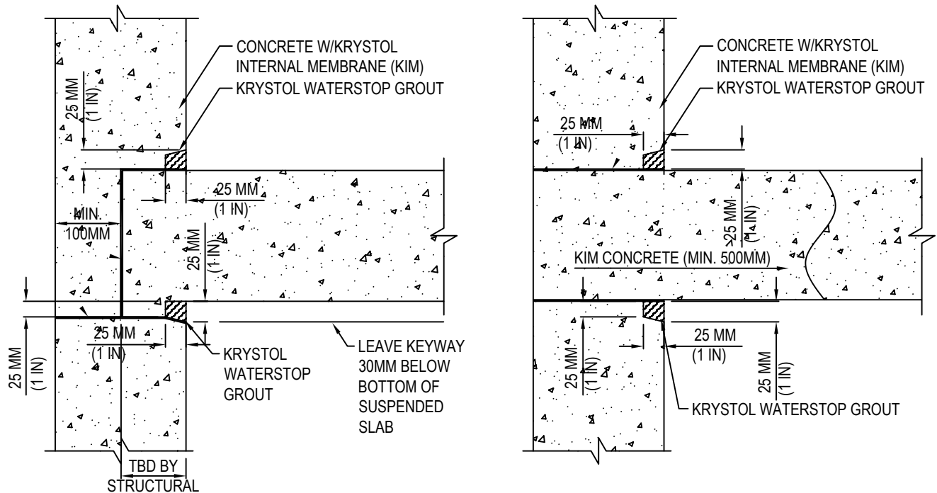
WALL TO ELEVATED SLAB CONTRUCTION JOINTS SINGLE PROTECTION; EXTERNAL GROUT METHOD
